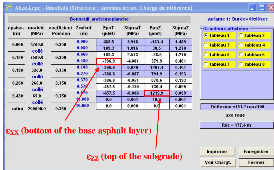
Figure 30 - Calculation of the critical strains using the Alizé-LCPC software
