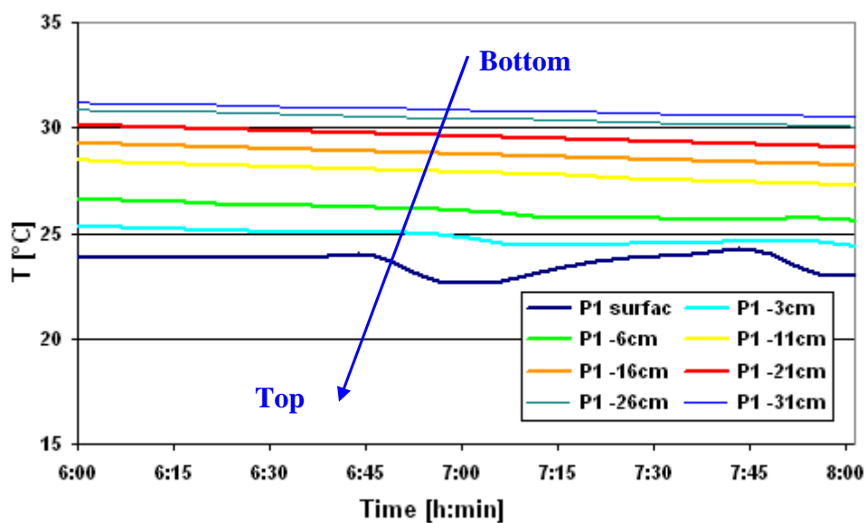
Figure 16 - Temperature in the asphalt layer during July 2 nd deep anchor experiment
