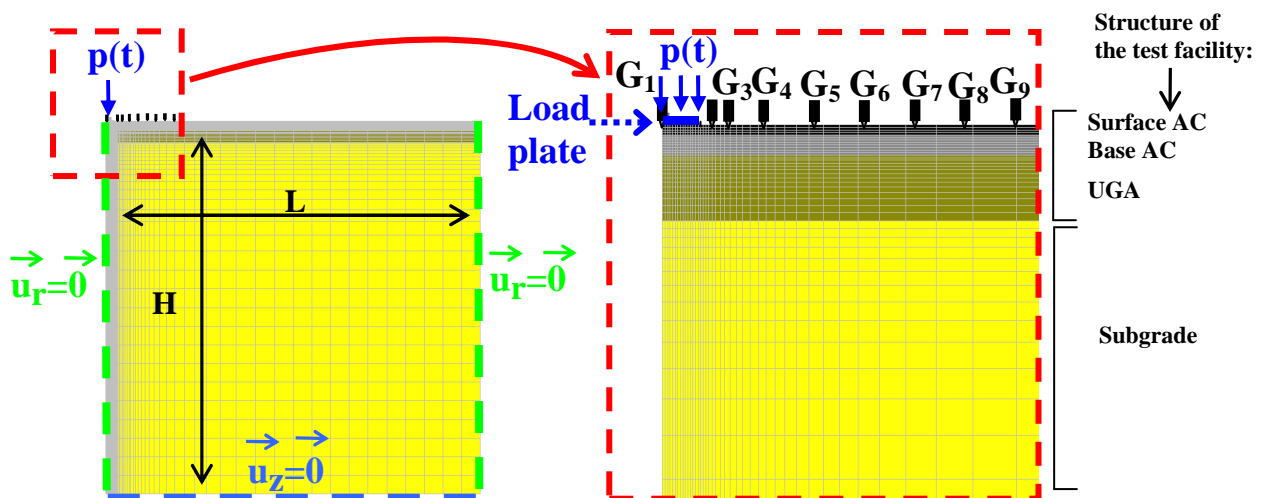
Fig. 2-1 The mesh
