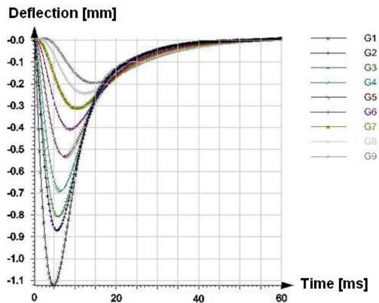
Fig. 3-25 Time-related deflections from M_1 modelling
