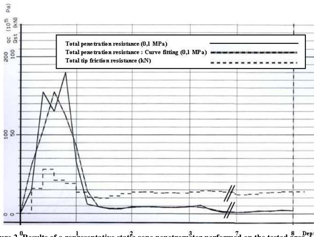
Figure 2- Results of a representative static cone penetrometer performed on the tested area.
