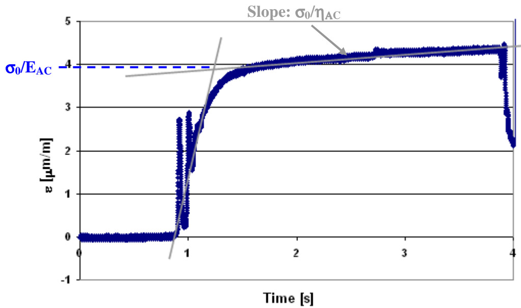
Fig. 1-52 Fitting of a Maxwell model on experimental results
