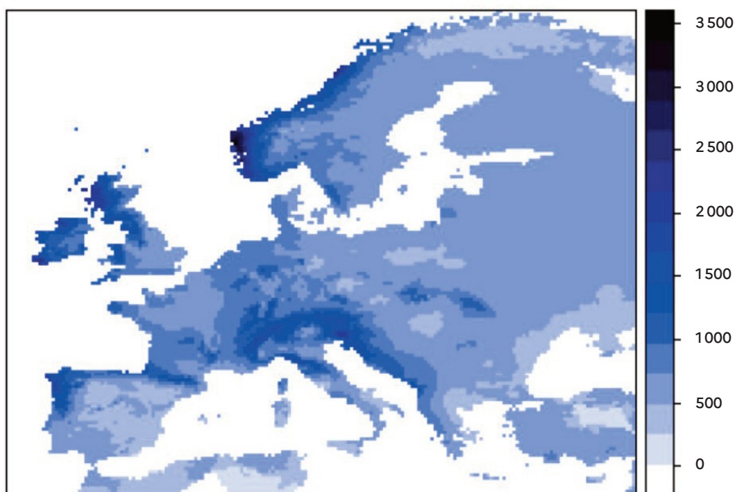
Figure 48 – Average annual precipitation in Europe. Data on a 17-year average (between 6 and 63 years depending on the station).
