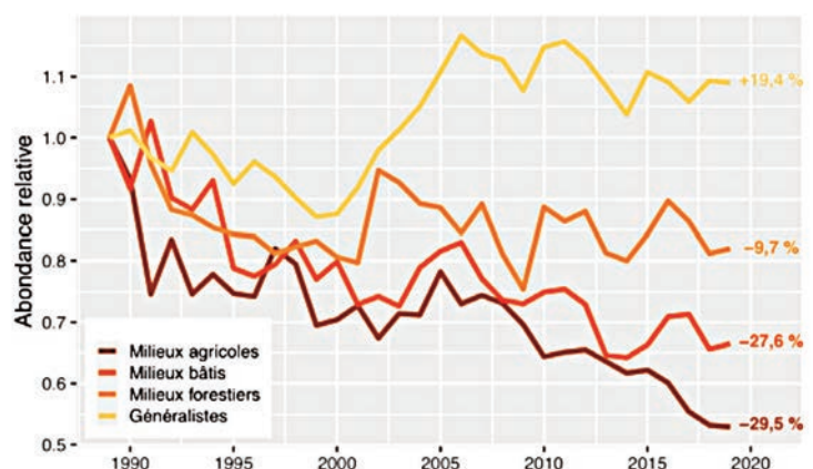
Figure 4 Evolution of indicators by group of birds' specializations.
