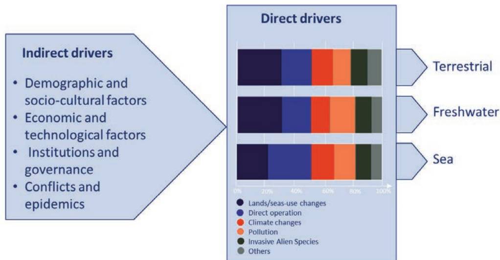
Figure 6 – Direct and indirect drivers of biodiversity decline.
