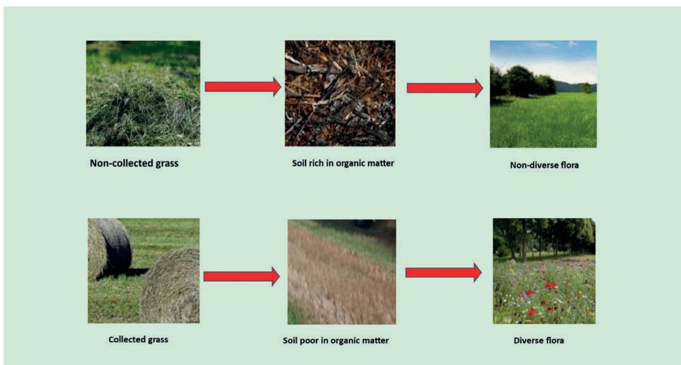
Figure 23 – The richness of biodiversity lies in the nutrient poverty of the soil.
